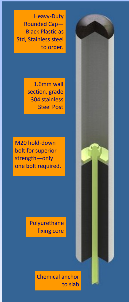
Sectional View
